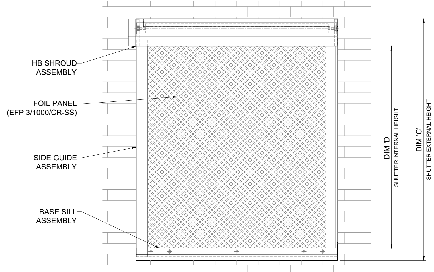
1 PLAN
