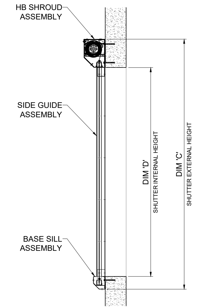
3 SECTION
