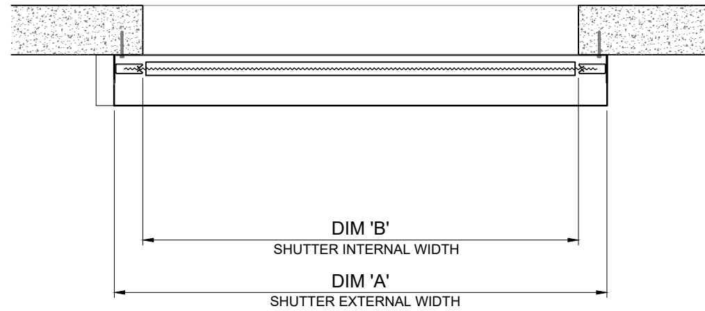
1 PLAN
