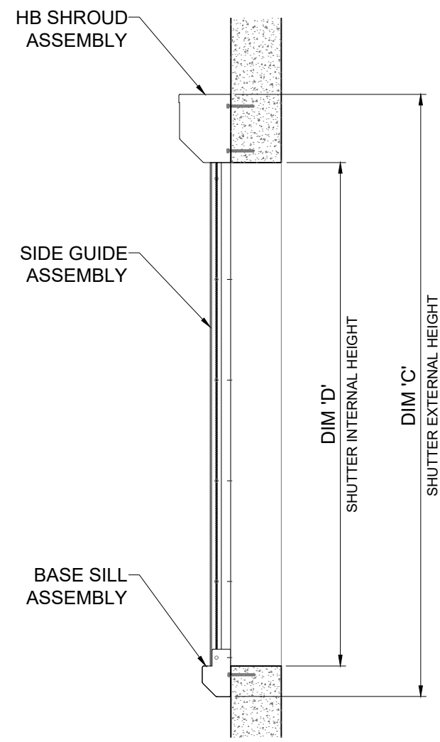
3 SECTION
